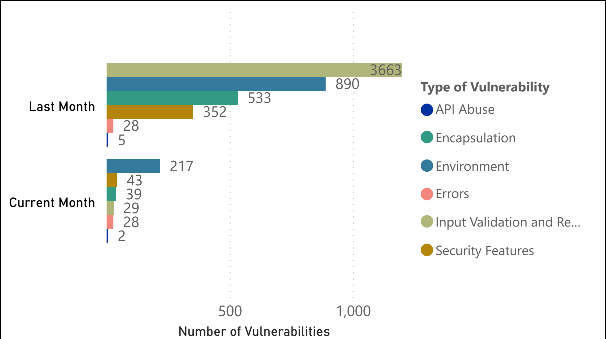
Vulnerability Type by Month
